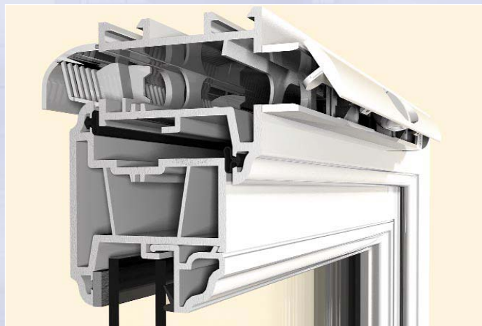
Overhead section
